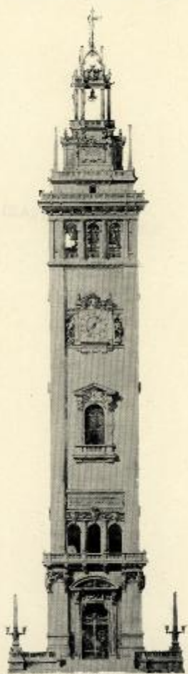
Design for the Clock Tower, Milan Cathedral (executed by the International Jury), LUCA BELTRAMI, Hon. Cons. Mem. R.I.B.A., Architect, Milan.
